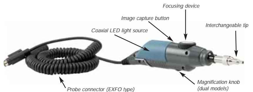
Probe connector (EXFO type)
