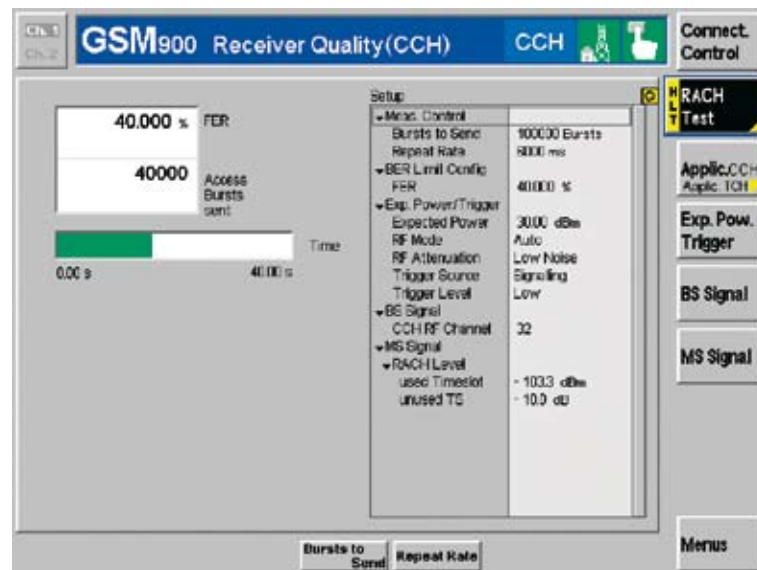
RACH test.
