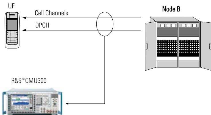
Setup for monitoring and logging.
