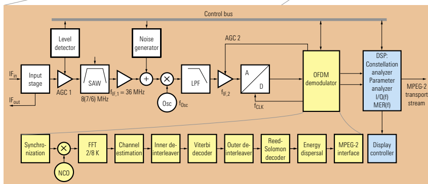
Block diagram of the R&S® EFA TV test receiver, models .40/43 (DVB-T)
