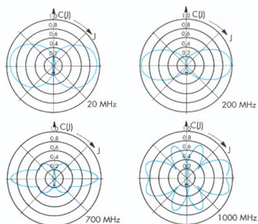
Elevation diagrams of Vertical Dipole HE309
