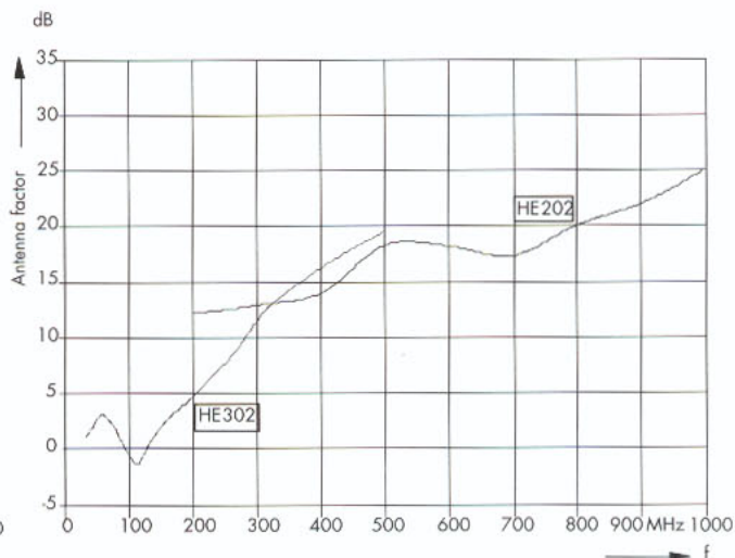
Antenna factor of Dipoles HE202 and HE302
