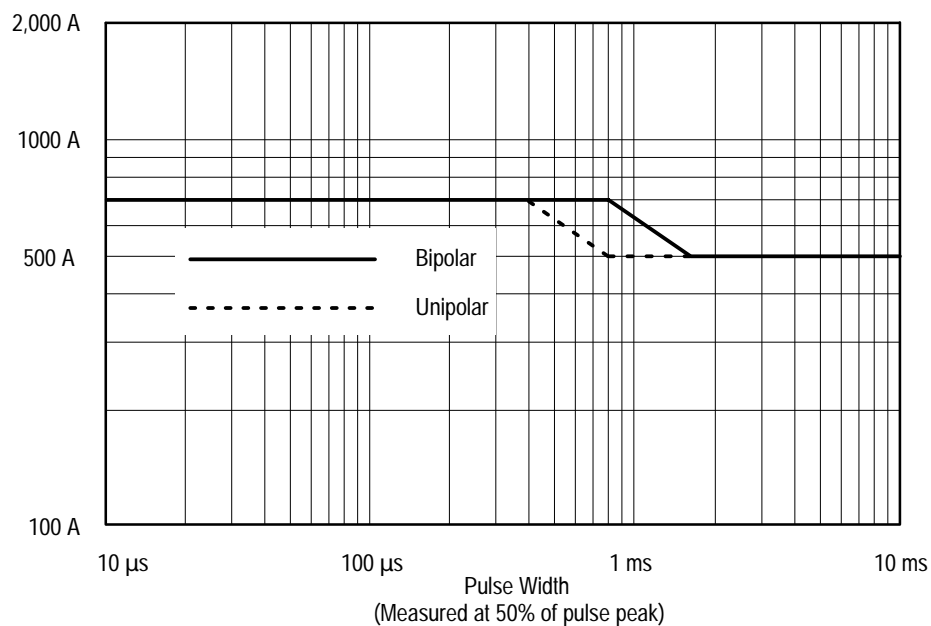
Figure 3: Typical Maximum Pulsed Current
