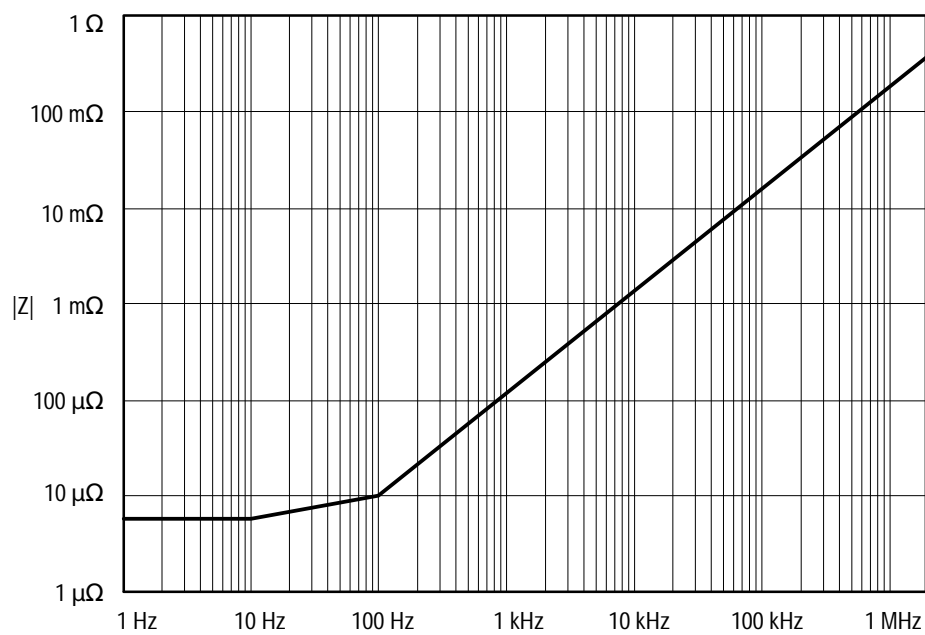
Figure 5: Typical Insertion Impedance Magnitude
