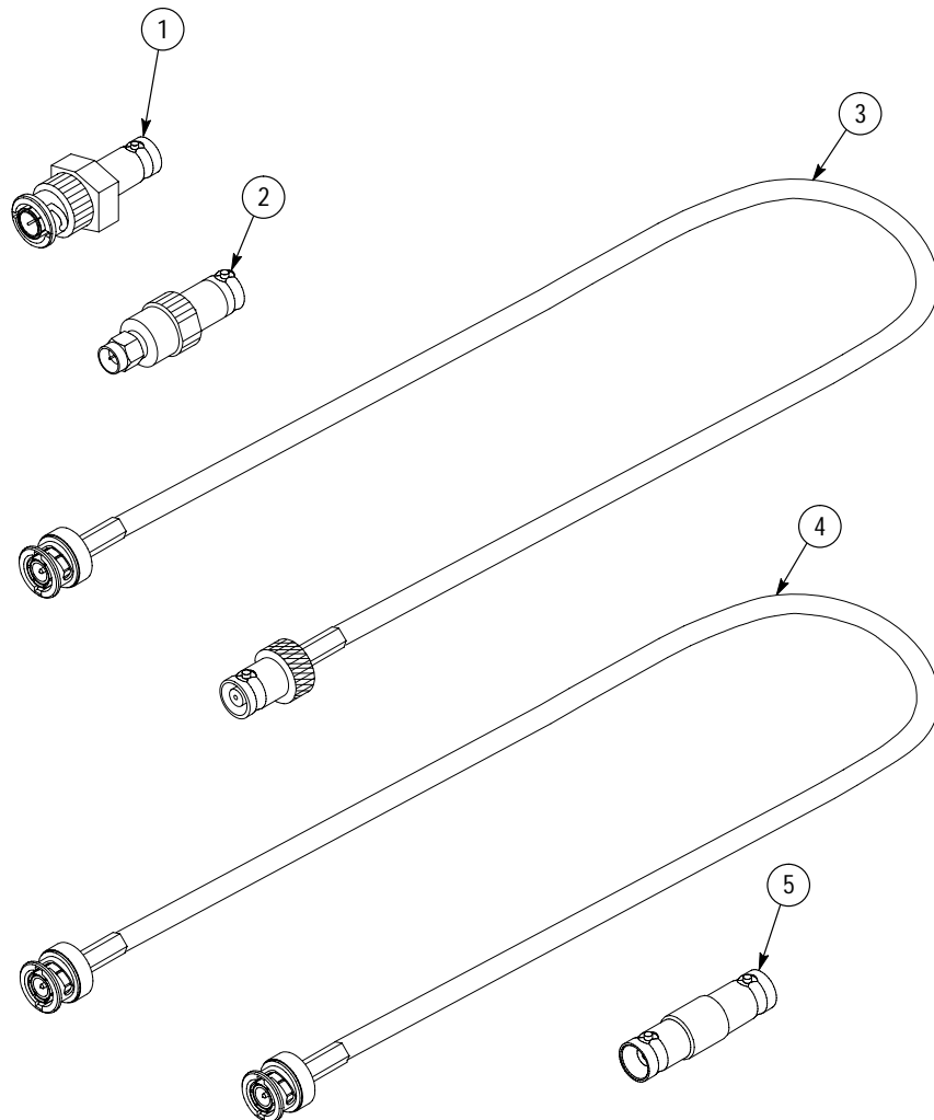
Figure 9: Optional accessories
