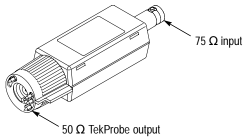
Figure 1: AMT75 Adapter
