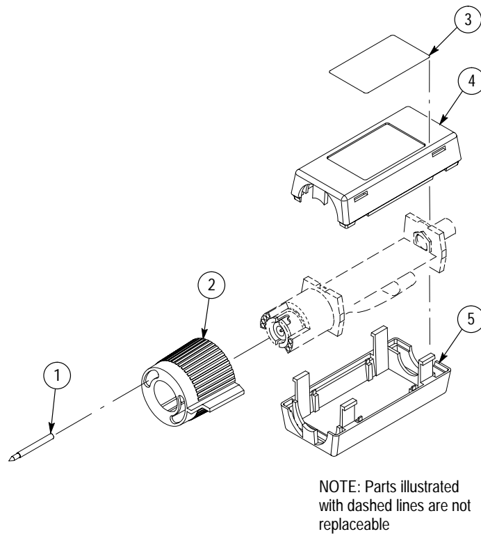
Figure 8: Replaceable parts
