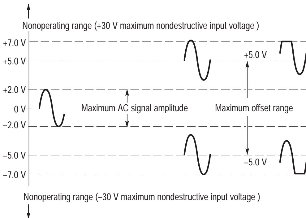
Figure 4: Dynamic and offset limitations
