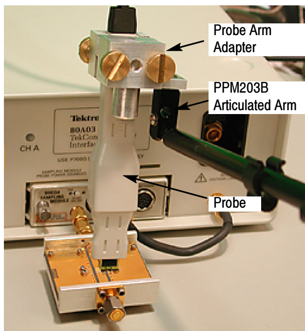
Figure 17: Fixtured Probe
