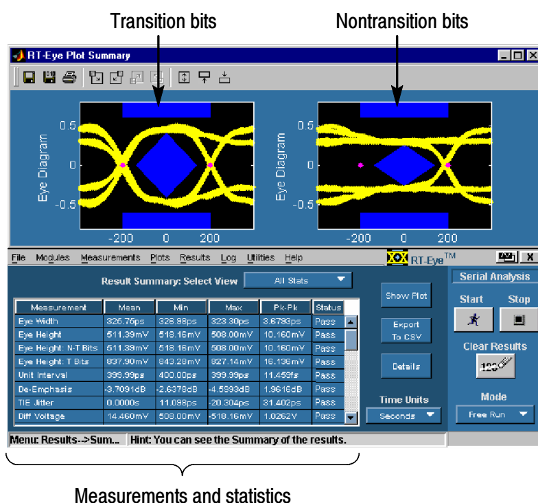
Figure 22: RT-Eye application
