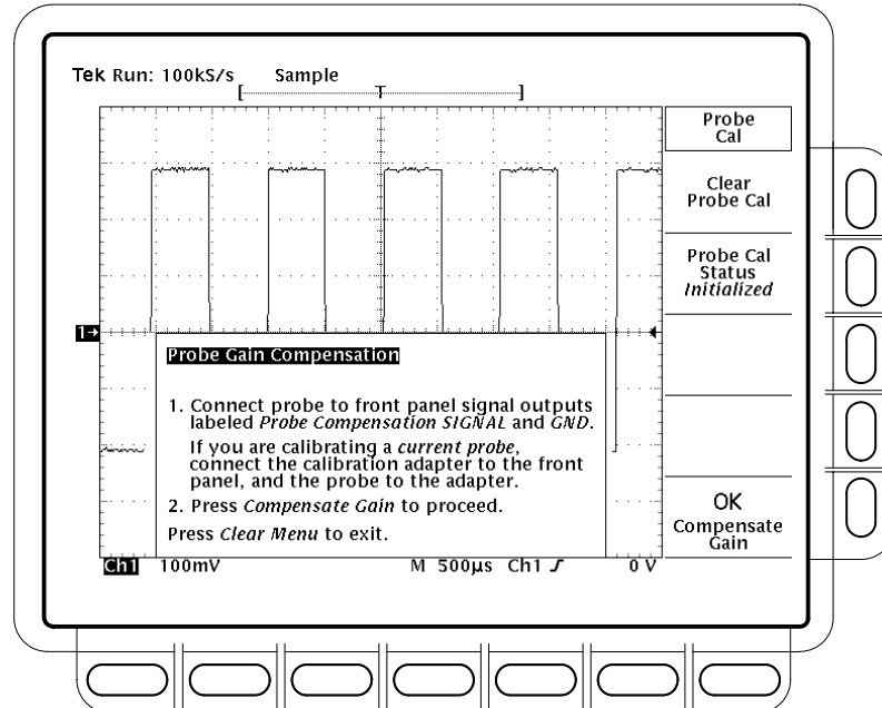
Figure 3–73: Probe Cal Menu and Gain Compensation Display
