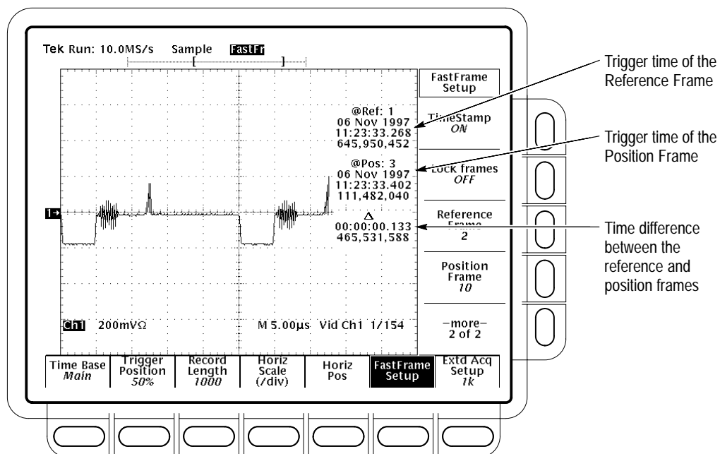
Figure 3-35: FastFrame TimeStamp
