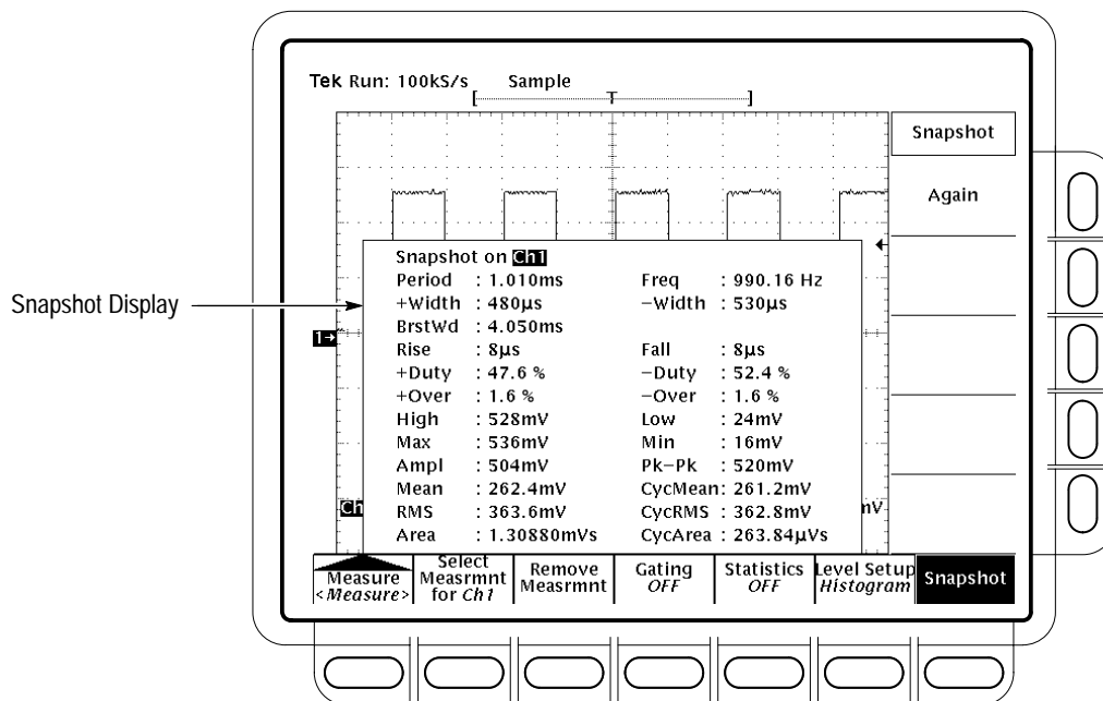
Figure 3-64: Snapshot Menu and Readout
