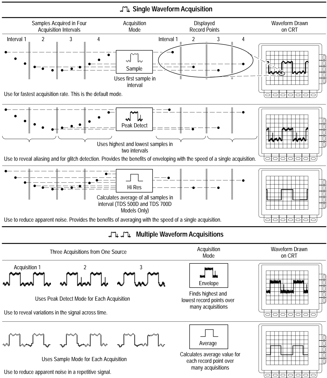
Figure 3–15: How the Acquisition Modes Work
