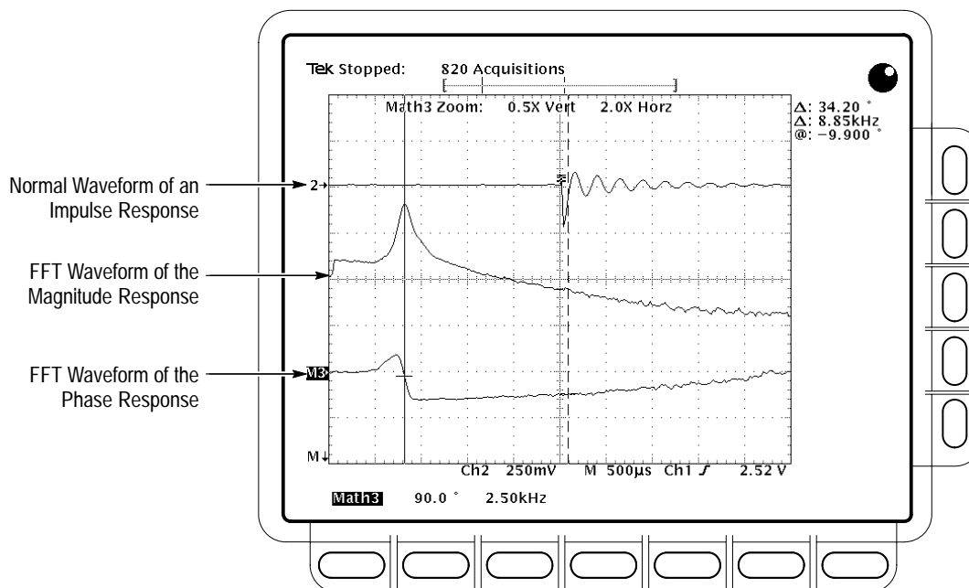
Figure 3-96: System Response to an Impulse
