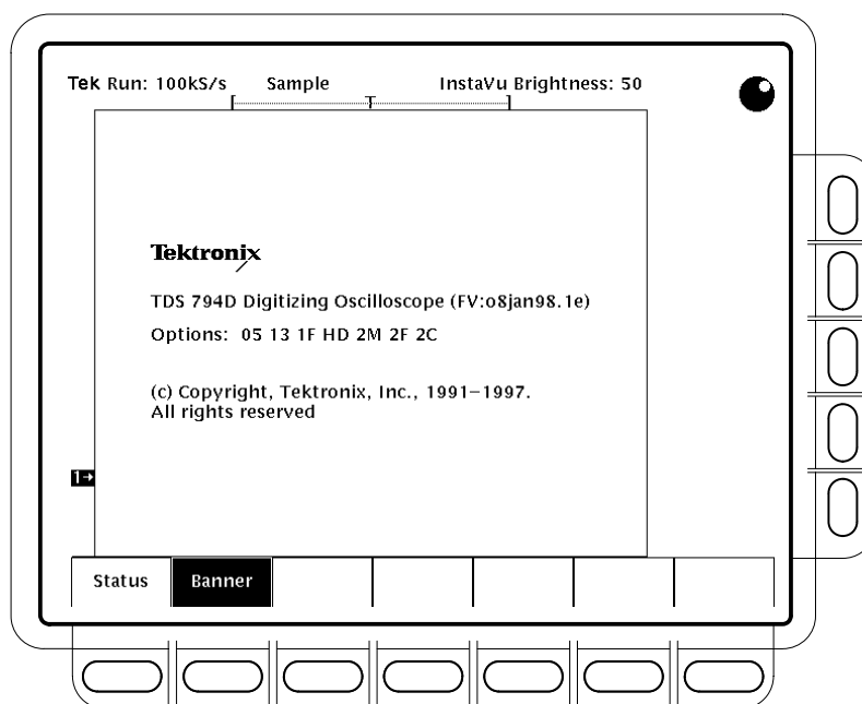
Figure 3–90: Banner Display
