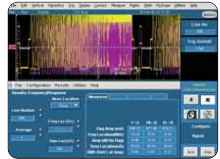
► Frequency Response Measurement Input Selections (Option SD and HD).
