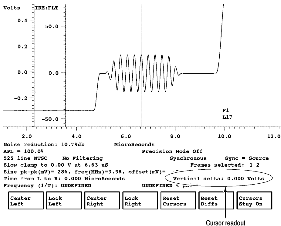
Figure 3-4: Color burst aligned with horizontal reference line
