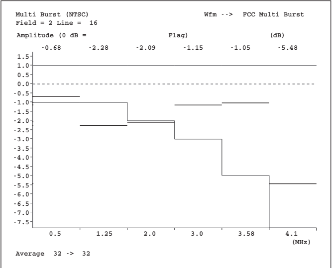
Multiburst measurement.
