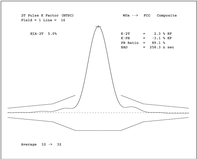
K-factor measurement.
