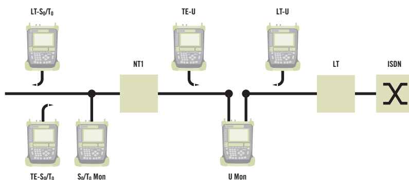
figure 1 Basic rate access
