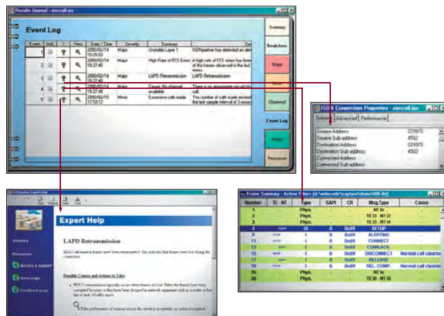
figure 7 Analysis with IBT-100/-200/-300 combined with ISDNpartner
