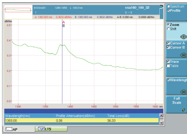
An attenuation profile showing a loss vs. wavelength measurement
