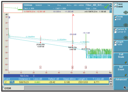
Pass/Fail analysis
