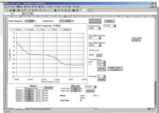
Phase noise measurement using sample software
