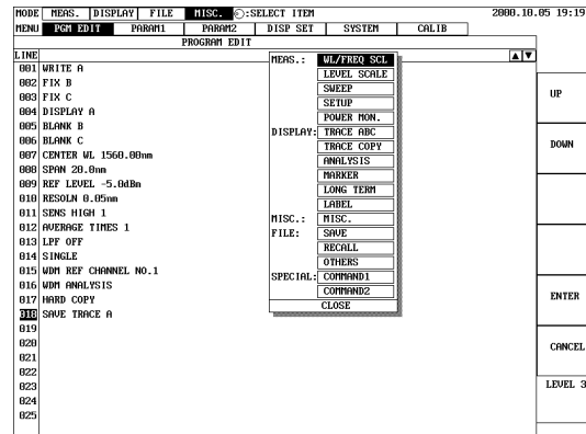
Programming example
