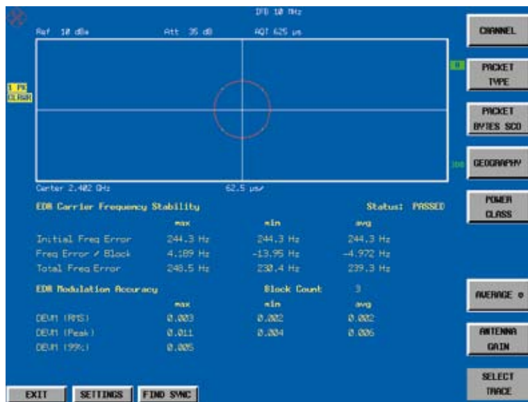
Measurement of initial carrier frequency tolerance of a Bluetooth® signal with R&S®FS-K8.
