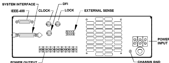
1503L REAR PANEL
