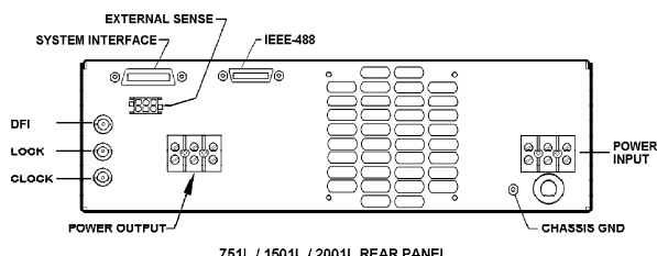
751L / 1501L / 2001L REAR PANEL
