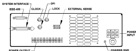
1503L REAR PANEL
