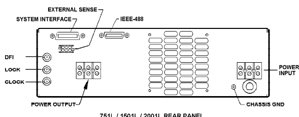
751L / 1501L / 2001L REAR PANEL
