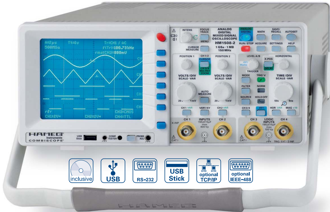
DSO mode: 4-channel display of 2 analog and 2 logic signals
