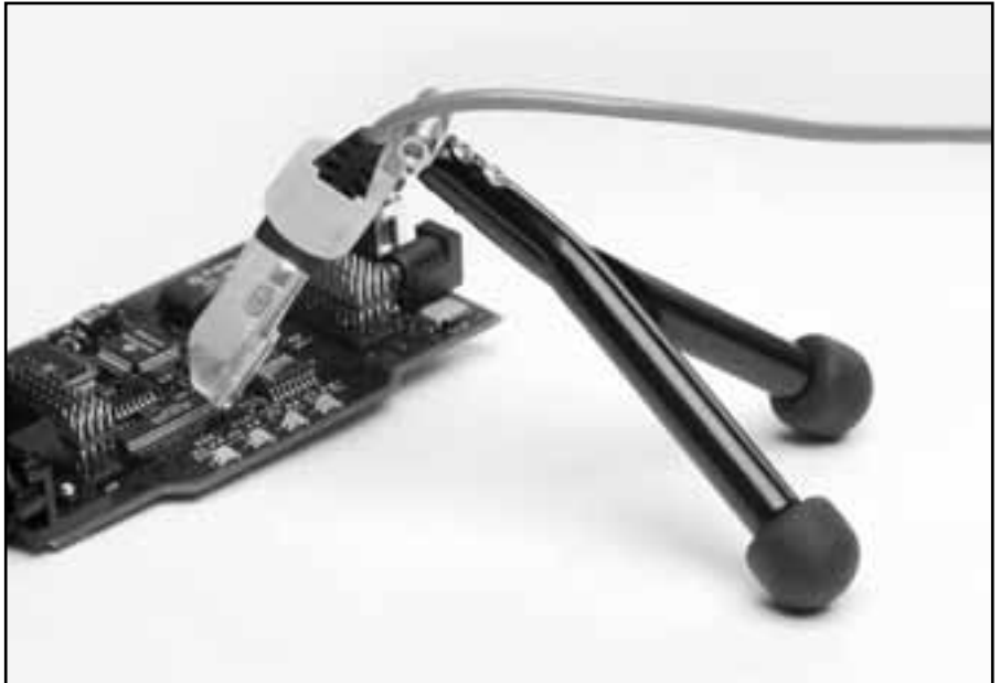
HFP probe with ingenious FreeHand probe holder.
