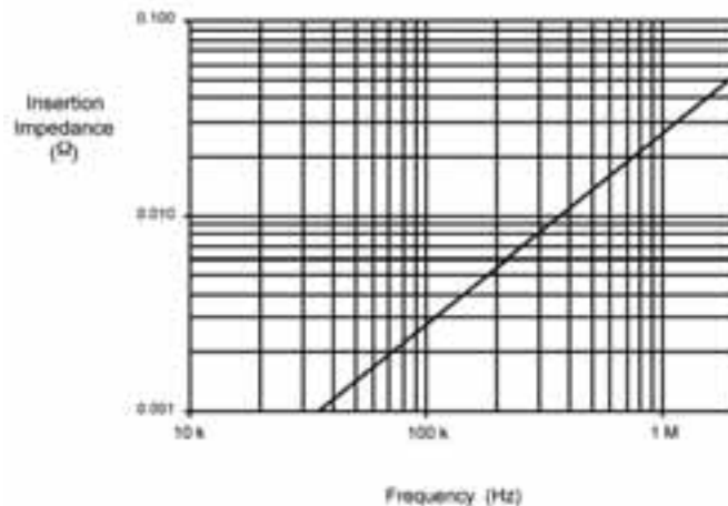
Insertion Impedance vs. Frequency
