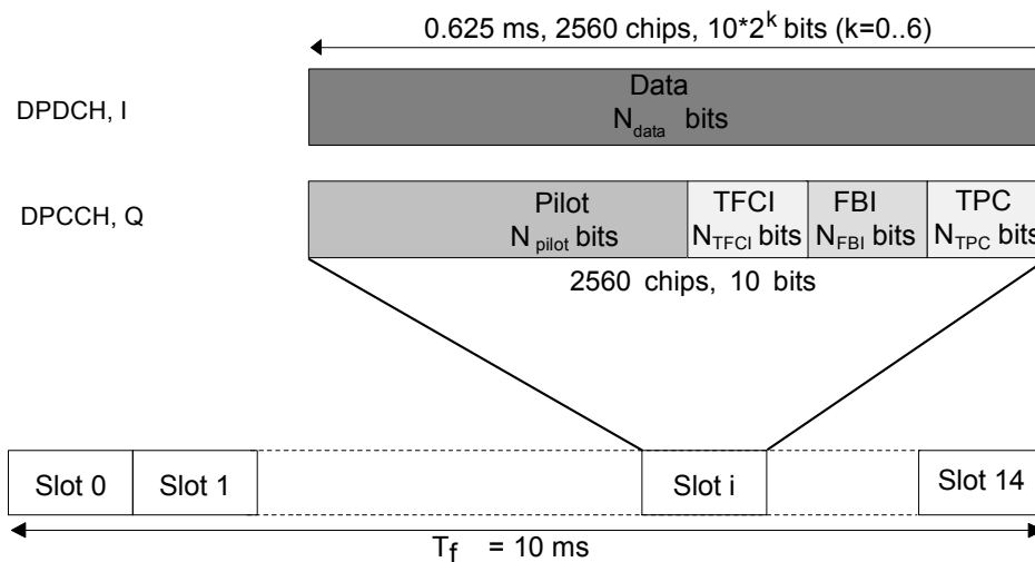
Fig. 4-37 Structure of an uplink DPCH in the time domain
