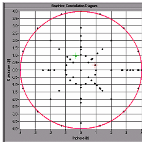
Fig. 4-23 Constellation diagram with clipping level 50 %, vector mode (i+j)
