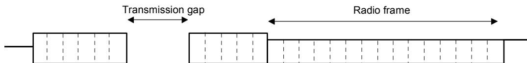
Fig. 4-35 Envelope of compressed mode signal with single-frame method
