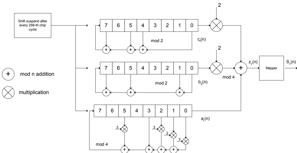
Fig. 4-18 Structure of uplink short scrambling code generator
