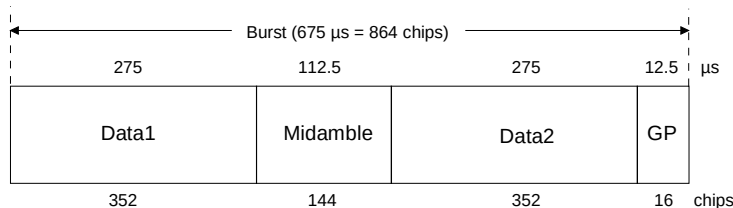
Fig. 4-1 Traffic burst without layer 1 control information
