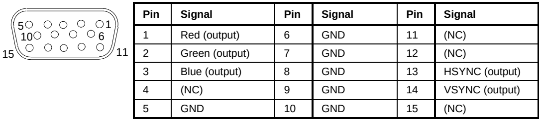
Figure 8-5 Pin assignment of the MONITOR connector
