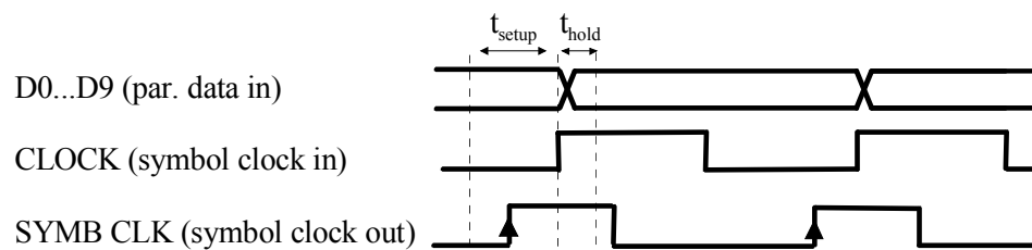
Fig. 4-15 External parallel data with high and low active external symbol clock. The setup time ( t_{\text{setup}} ) and hold time ( t_{\text{hold}} ) can be found in the data sheet.
