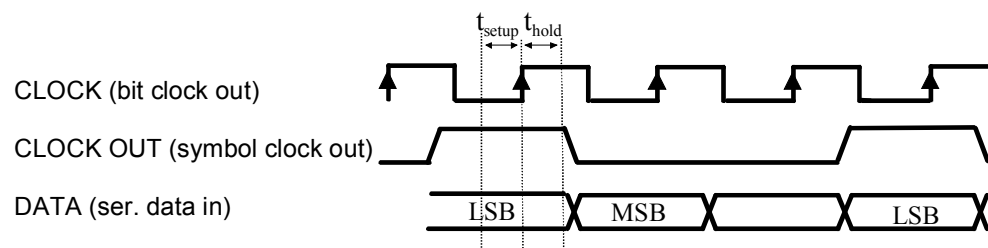
Fig. 4-12 External serial data and the clock signals which are output (bit clock and symbol clock). The setup time ( t_{\text{setup}} ) and hold time ( t_{\text{hold}} ) can be found in the data sheet.
