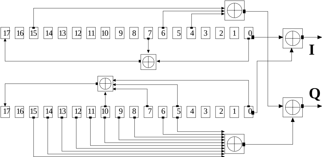
Fig. 4-19 Structure of downlink scrambling code generator
