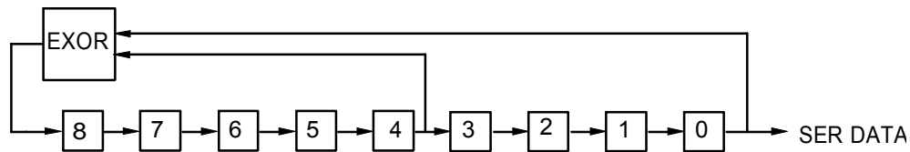
Fig. 4-9 9-bit PRBS generator
