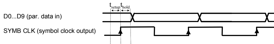
Fig. 4-13 External parallel data, internal clock signal and the clock signal that is output on the AUX I/O interface. The setup time ( t_{\text{setup}} ) and hold time ( t_{\text{hold}} ) can be found in the data sheet.
