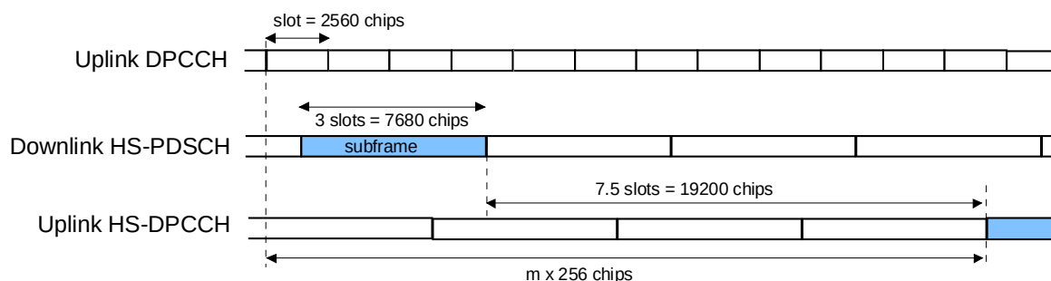
Fig. 4-41 Timing offset between the uplink DPCCH, the HS-PDSCH and the HS-DPCCH at the UE.
