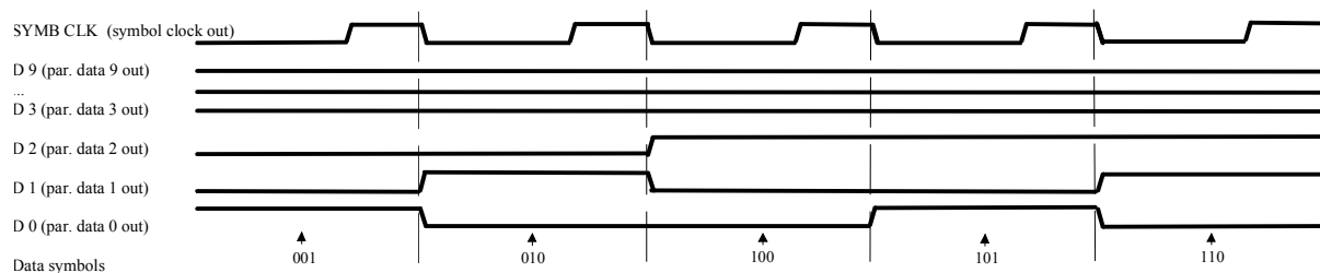
Fig. 4-11 Data and clock output signals on the parallel AUX I/O interface
