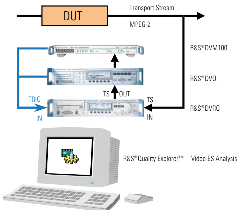
Error analysis with R&S®DVRG and realtime analyzers
