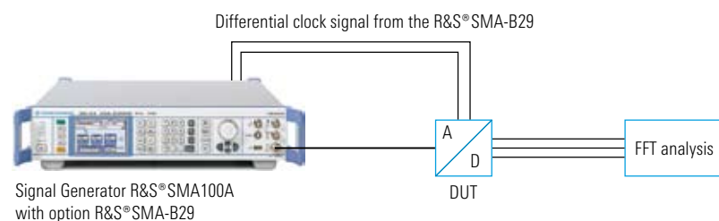
Application example: A/D converter test with the R&S®SMA100A
