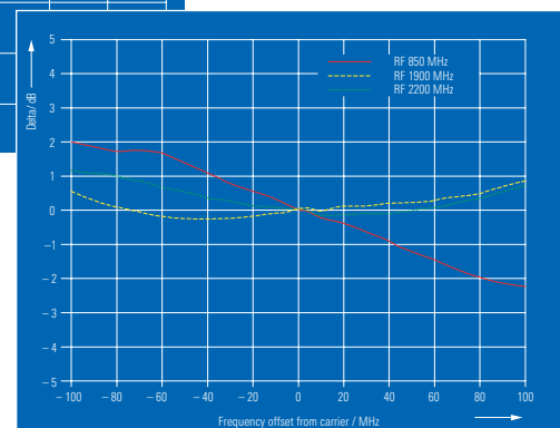
Frequency response (mode: external wideband I/Q)
