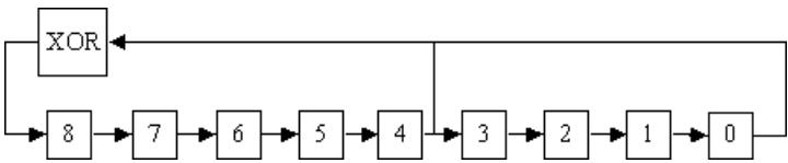
Fig. 2–9 The following table lists the generator data for the types of PRBSs implemented in WinIQOFDM. The initial state is always a 1 in register No. 0, and 0 in all other registers. According to CCITT V.52, the output bits of some PRBS generators are inverted. Since all PRBSs in this table are designed to have maximum length, their lengths are given by
