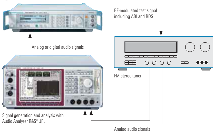
Signal Generator R&S®SML+Stereo/RDS Codec R&S®SML-B5
