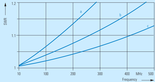
Typical SWR of a matched 50 \Omega line after connecting the RF Probe R&S®URV5-Z7 (without adapter, short ground connection); a) direct, b) with 20 dB plug-on divider, c) with 40 dB plug-on divider
