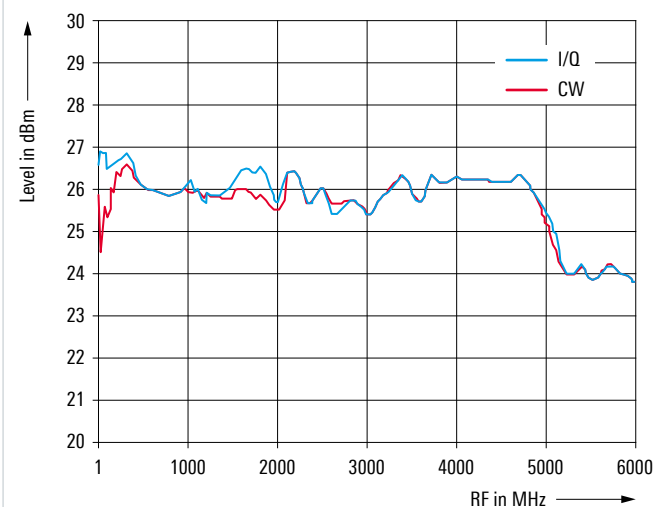
Measured maximum output power vs. frequency
