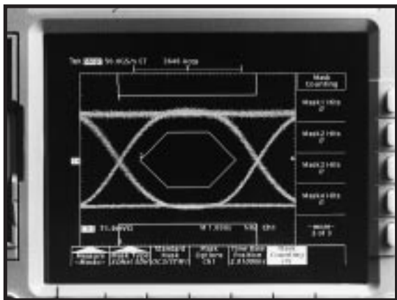
A SONET/SDH (OC-3/STM-1) signal is compared with the standard mask, showing a compliant waveform.
