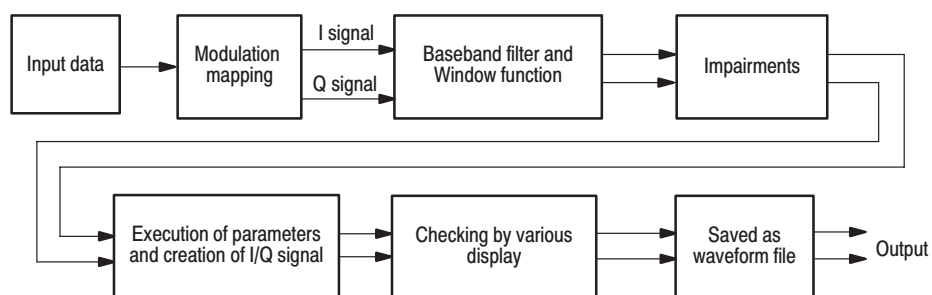
Figure 3-49: Outline flow for producing digital modulation waveform
