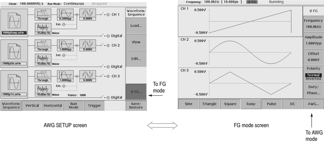
Figure 3-93: Change the generator mode (AWG430)
