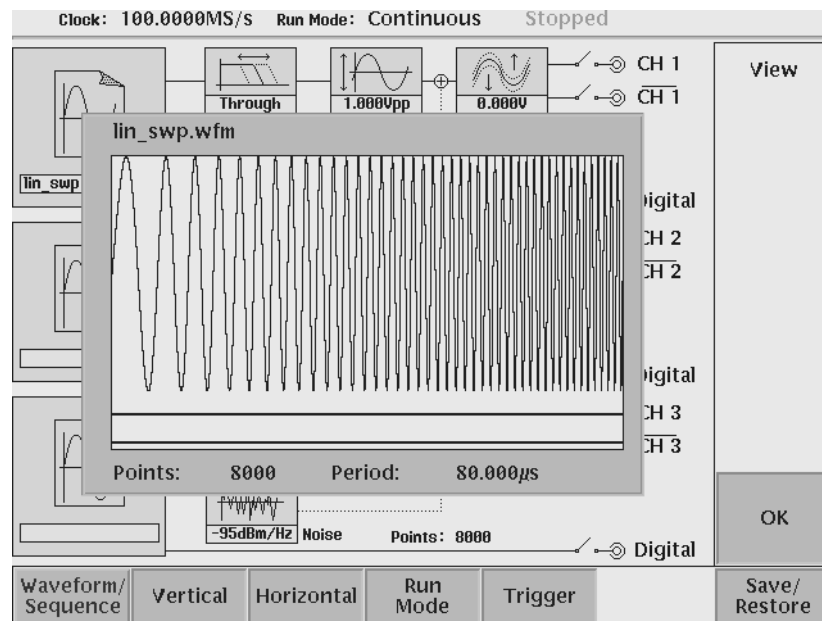
Figure 2–37: Viewing a waveform loaded into memory
