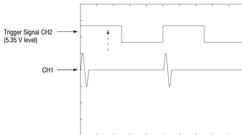
Figure B-26: Trigger Signal (+5V check2)
