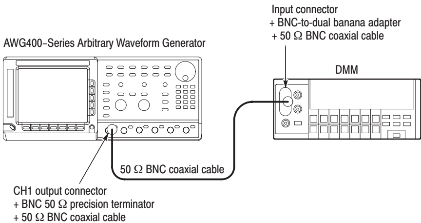
Figure B-16: Amplitude accuracy initial test hookup
