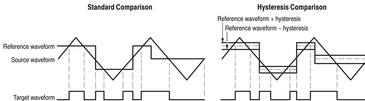
Figure 3–9: Waveform compare operation example
