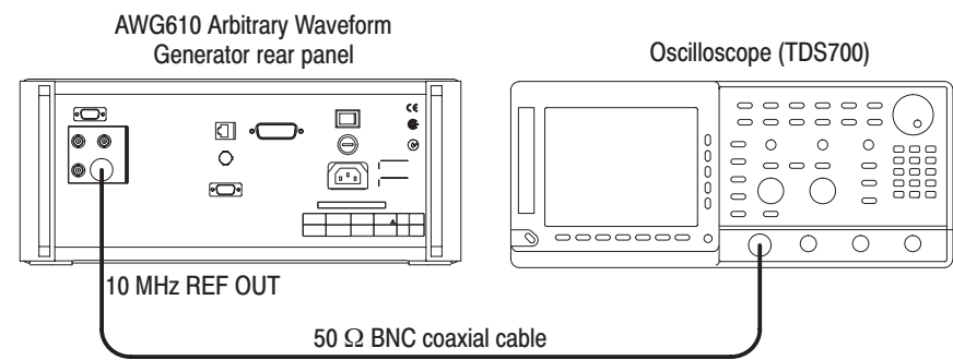
Figure B-30: 10MHz Reference output level initial test hookup
