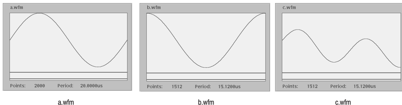
Figure 3–59: Waveforms generated from the Example 1 equation
