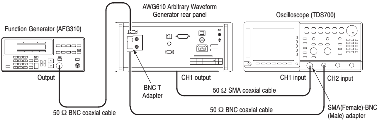
Figure B-15: Trigger input initial test hookup
