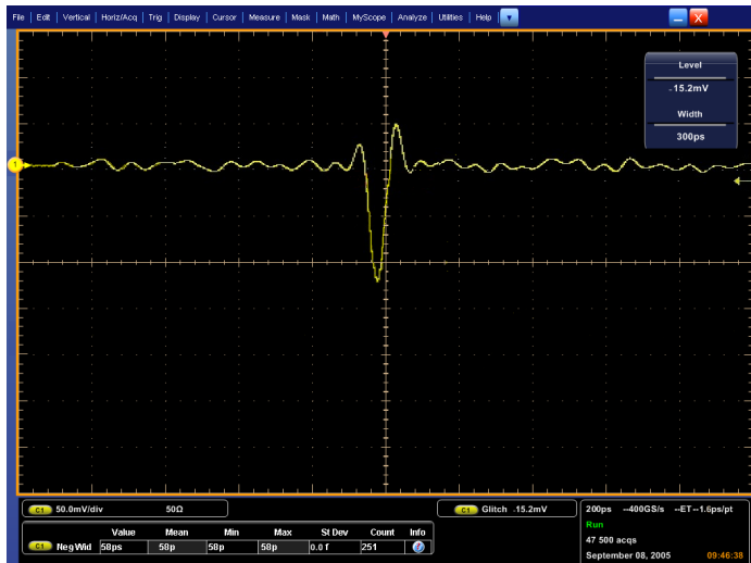
Pinpoint triggering can isolate glitches down to 100-ps wide
