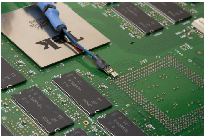
Low-cost solder tip features quick connection so moving probe to various solder points is fast and easy
