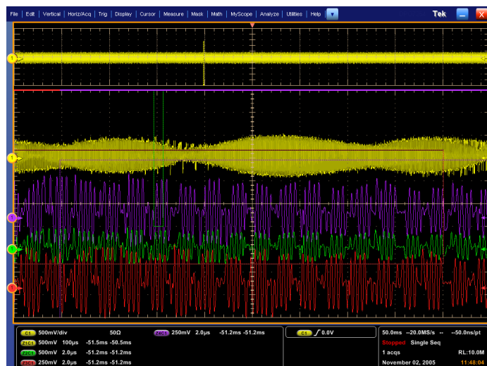
Zoom in on four areas of interest simultaneously to quickly compare them
