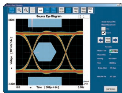
► HDMI compliance testing.
