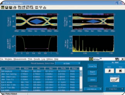
► FB-DIMM compliance testing.
