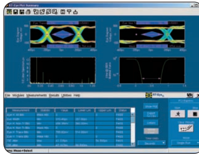
► RT-Eye® version 2.0 – PCI Express Rev1.1 Compliance test.
