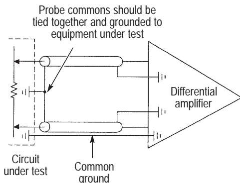
Figure 2-2: Optimizing high-frequency CMRR performance
