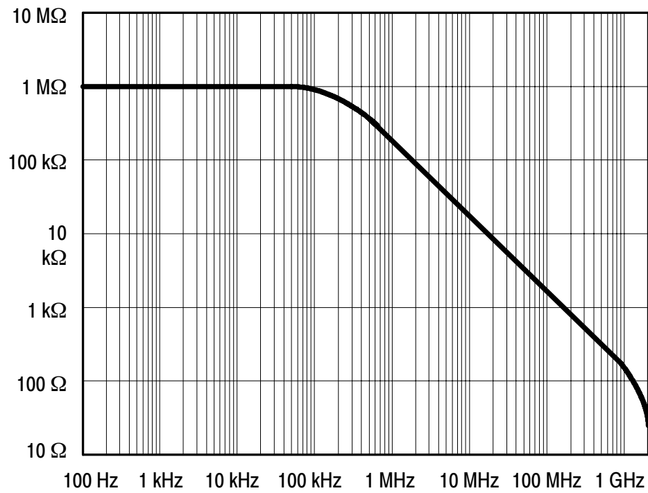
Figure 9: Typical Input Impedance vs. Frequency
