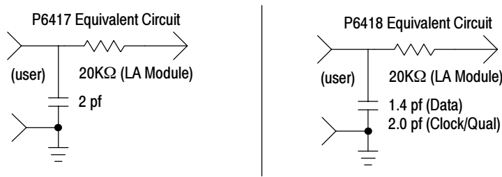
Figure 7: Probe loading
