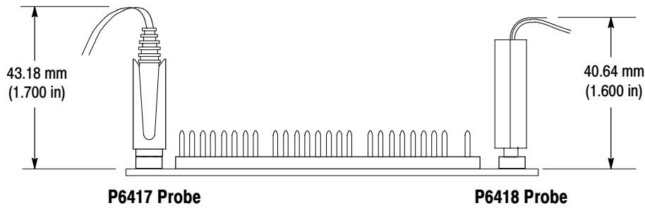
Figure 6: Probe podlet clearance
