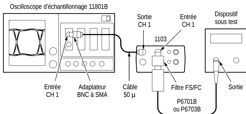
Figure 4: Installations sans l'interface TekProbe II
