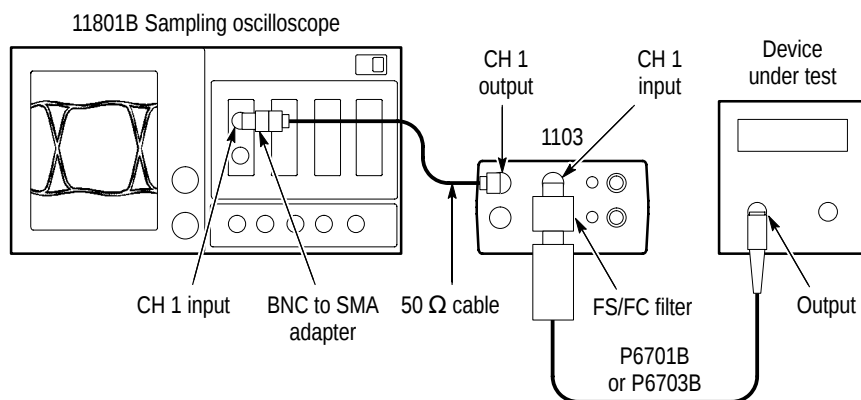
Figure 4: Setups without the TekProbe II interface
