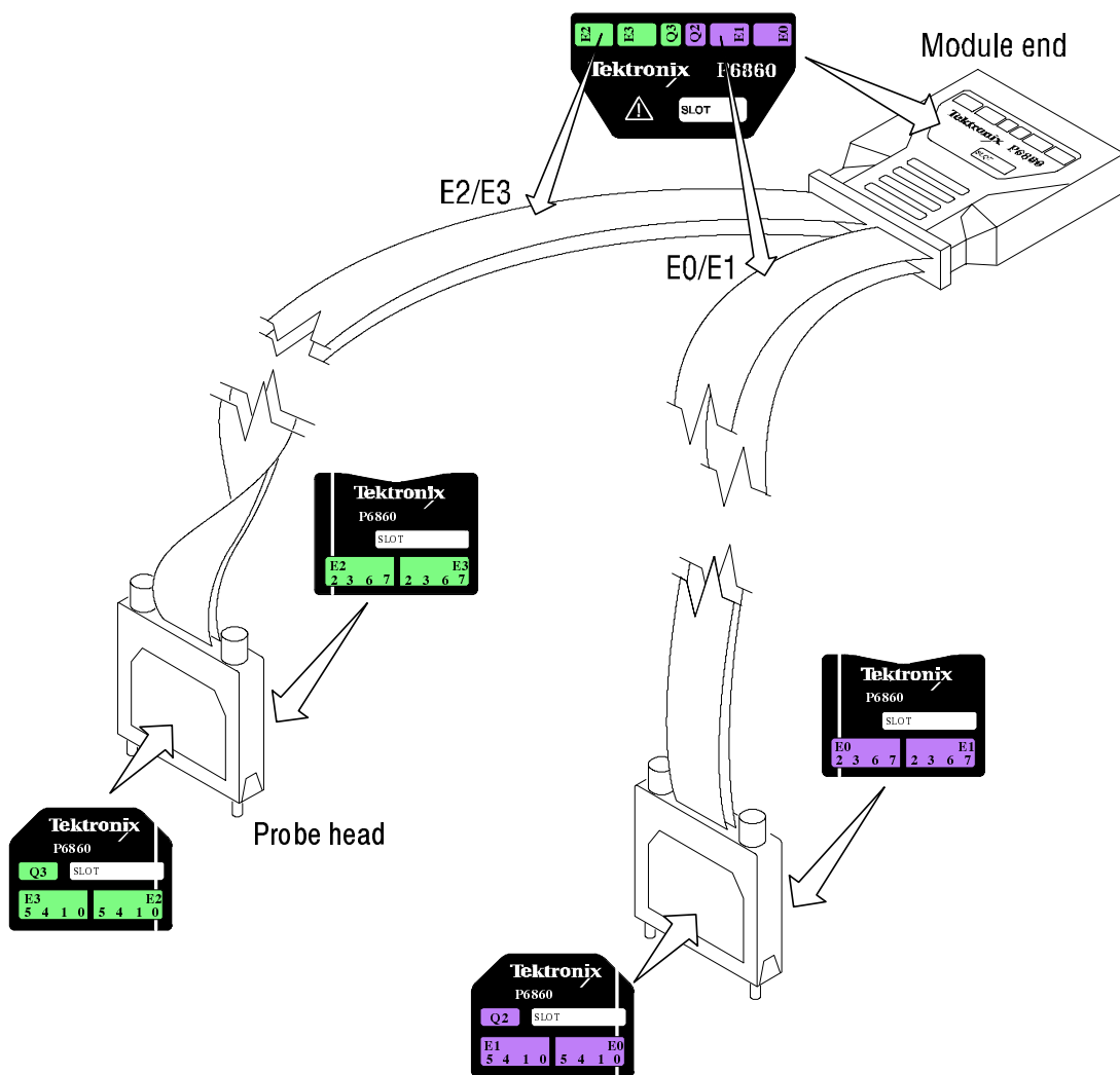
Figure 2: Attaching the P6860 High Density probe labels
