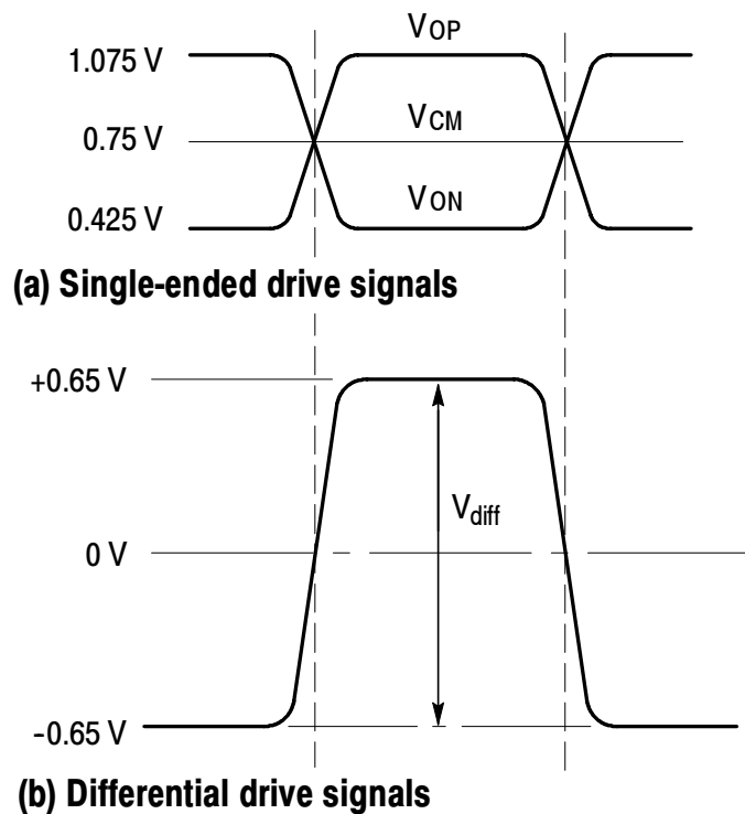
Figure 27: InfiniBand signals
