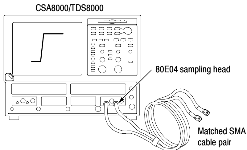
Figure 24: Checking skew between inputs
