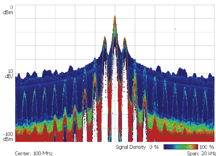
Figure 2-44: Persistence display
