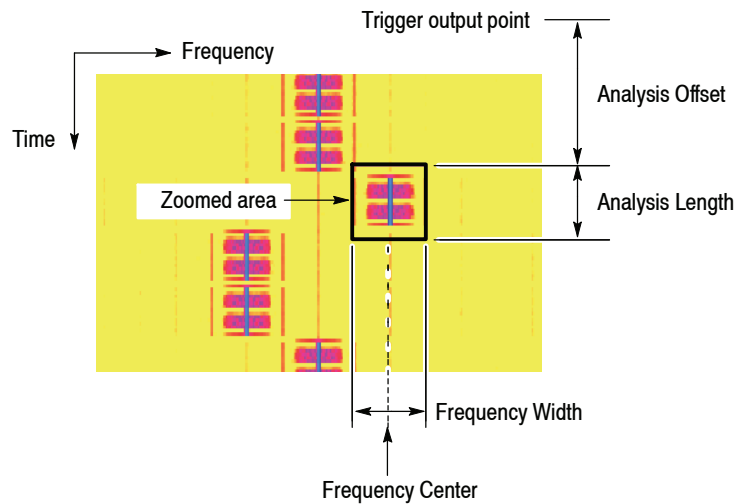
Figure 3-28: Zoom domain settings using the Acquisition/Analysis menu
