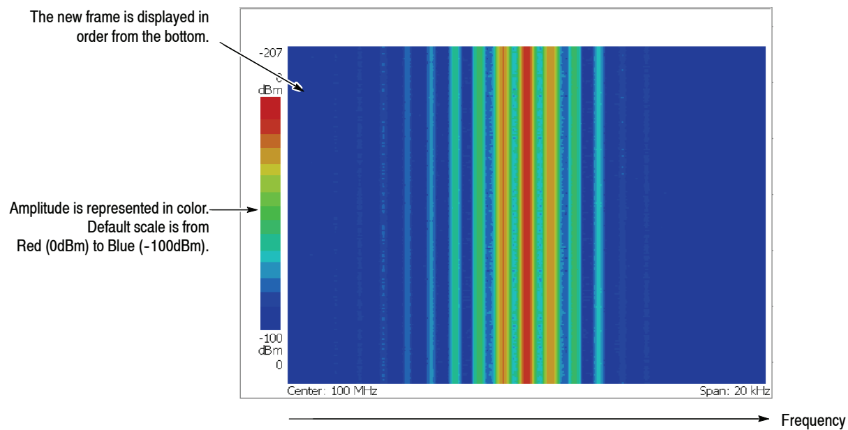
Figure 2-47: Spectrogram view
