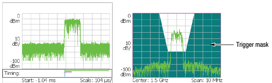
Figure 3-119: Trigger mask
