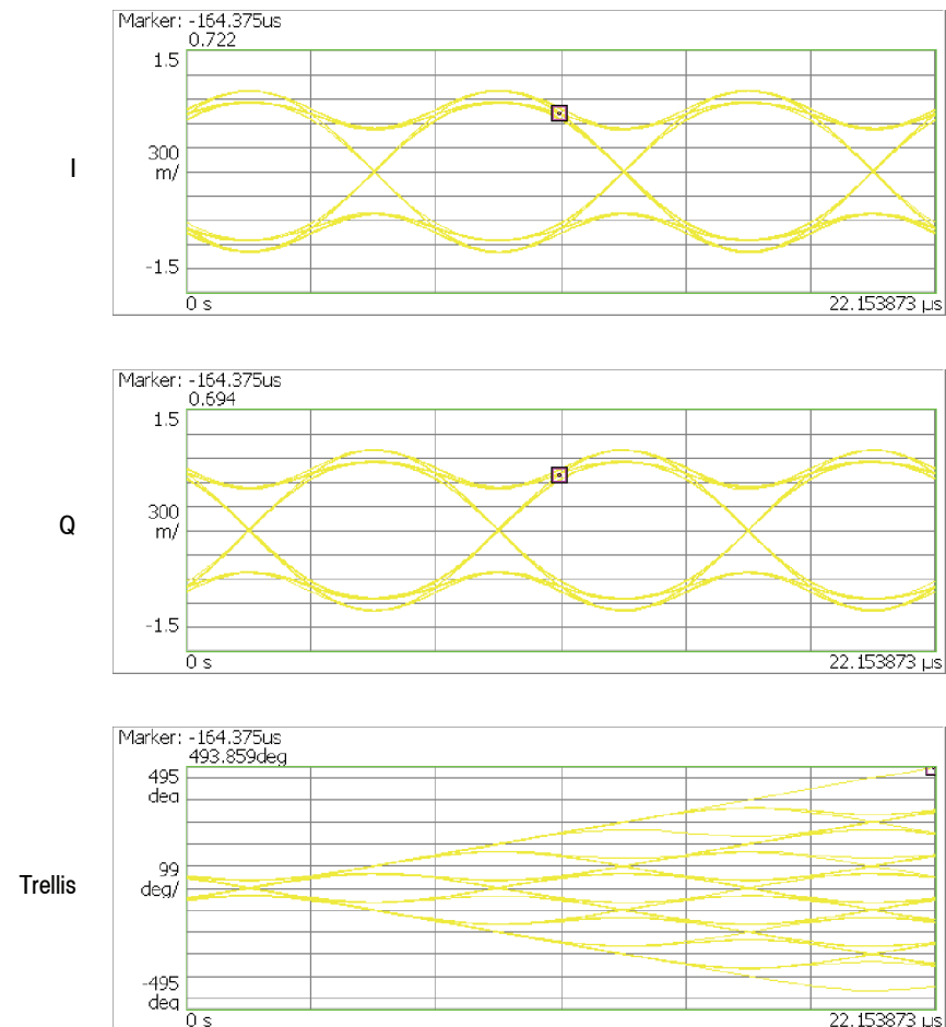
Figure 3-152: Eye diagram view
