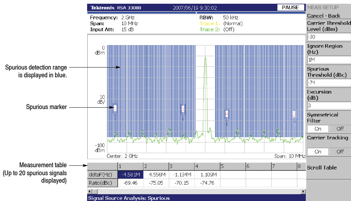
Figure 3-88: Spurious measurement
