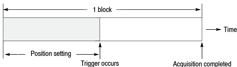
Figure 3-115: Trigger position
