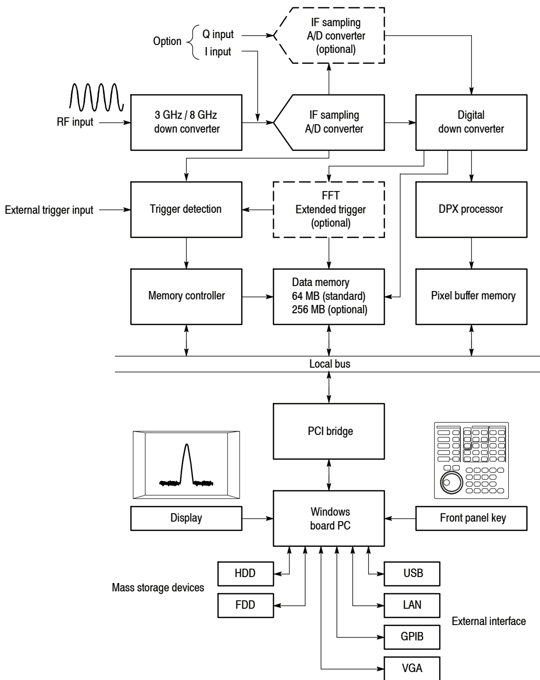
Figure 1-8: Block diagram
