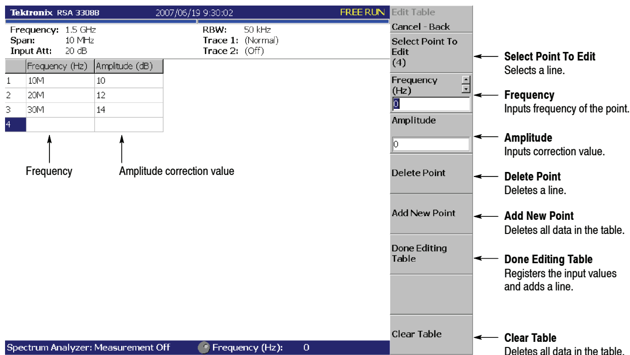
Figure 3-105: Amplitude correction data input
