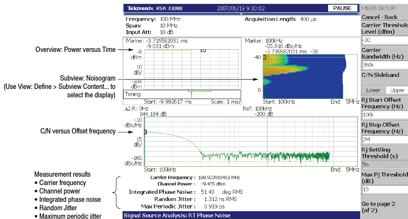
Figure 3-90: Real-time phase noise measurement
