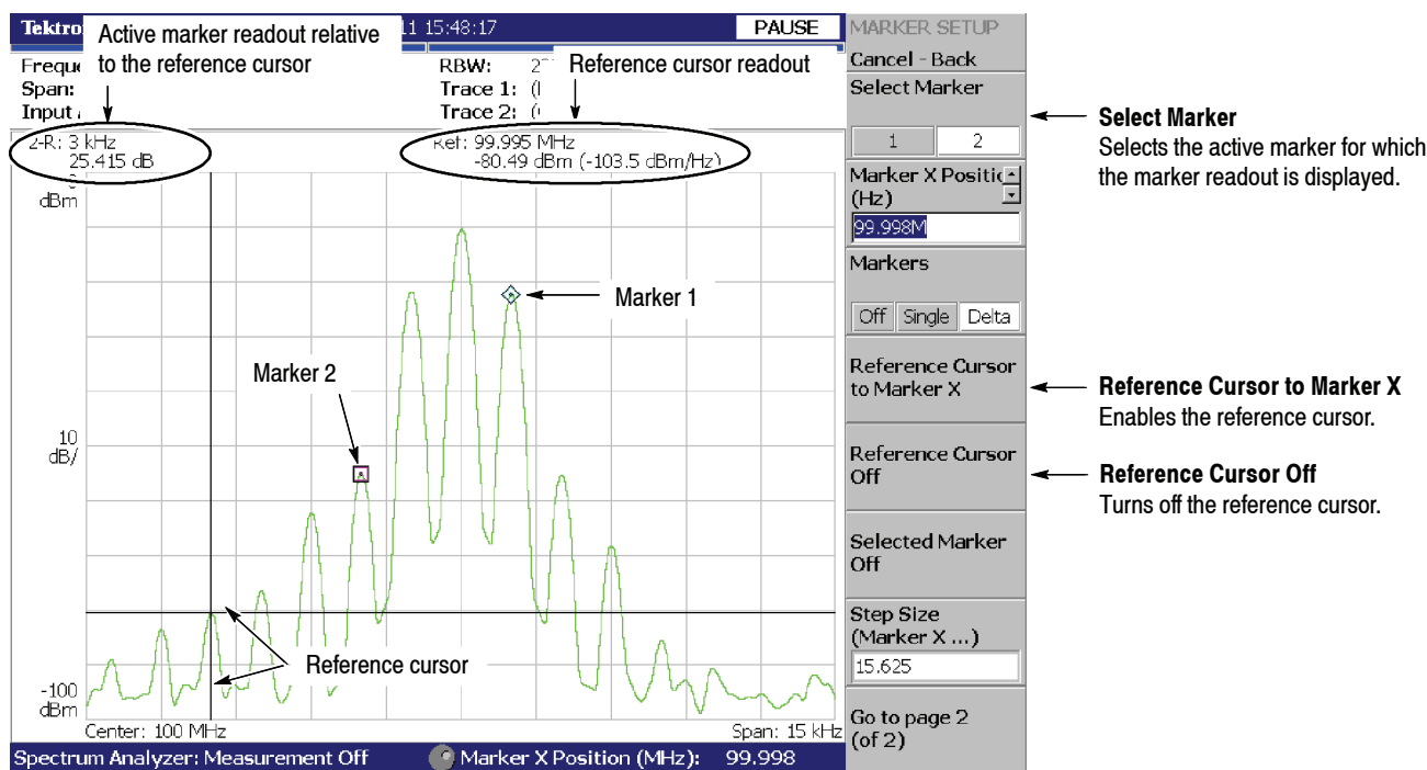
Figure 3- 167: Measurement with the reference cursor
