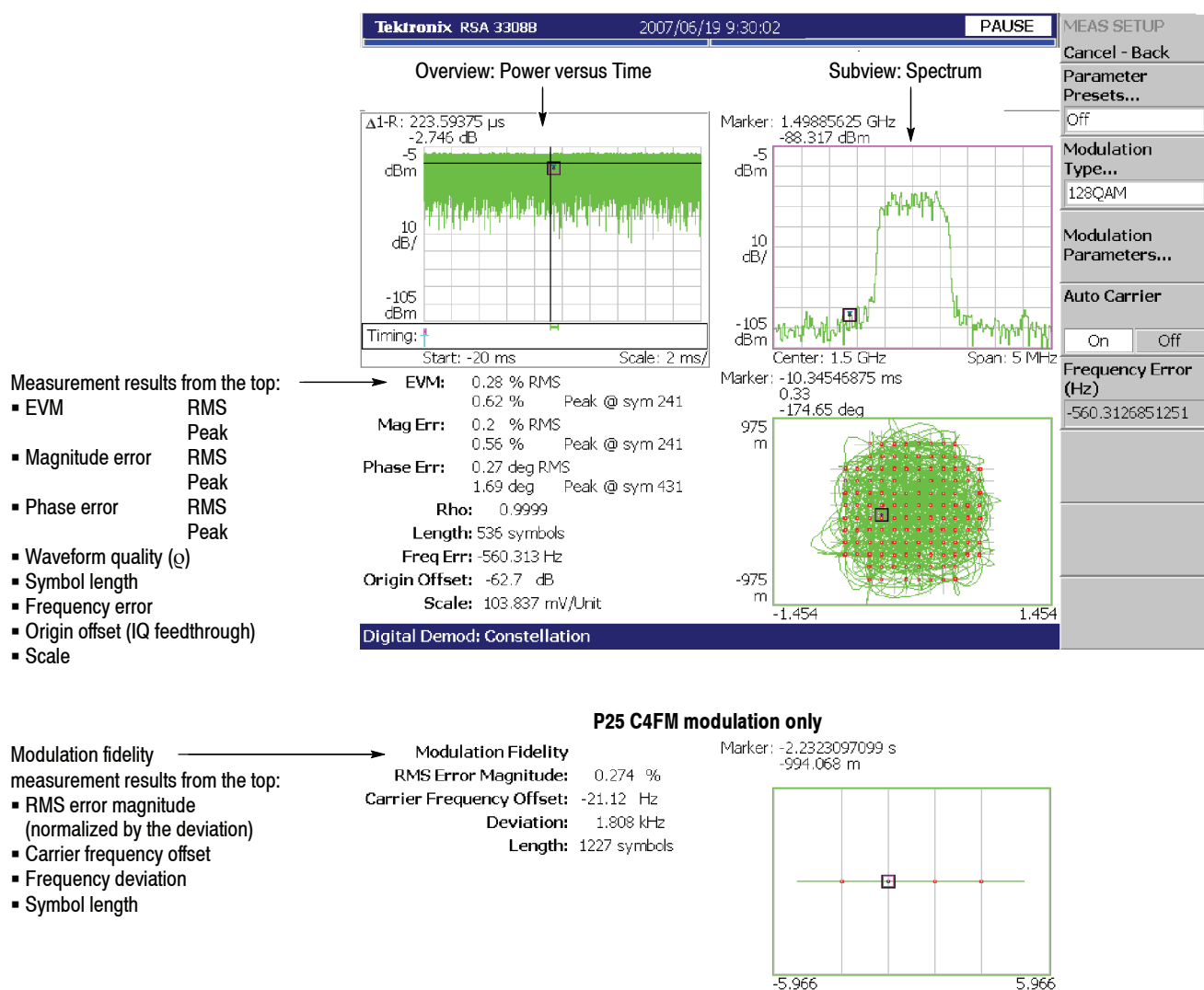
Figure 3-45: Constellation analysis
