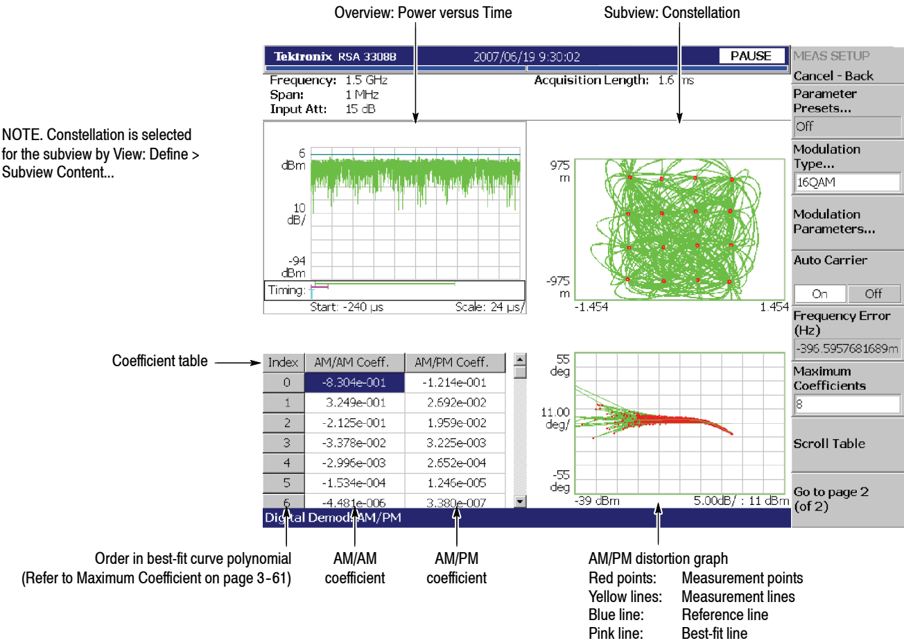
Figure 3-53: AM/PM measurement
