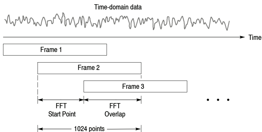
Figure 3-131: FFT overlap
