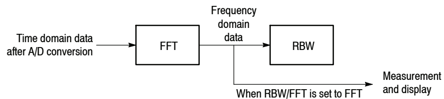
Figure 3- 130: Process flow when RBW/FFT = FFT
