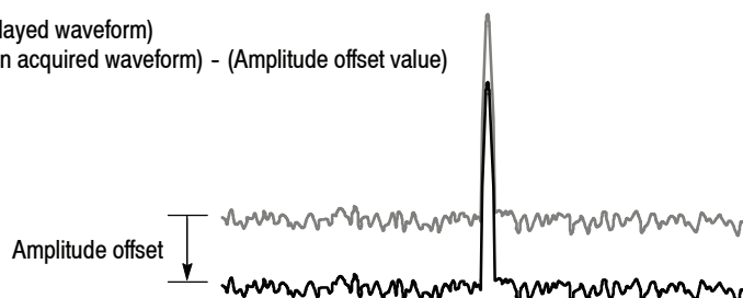
Figure 3-106: Amplitude offset
