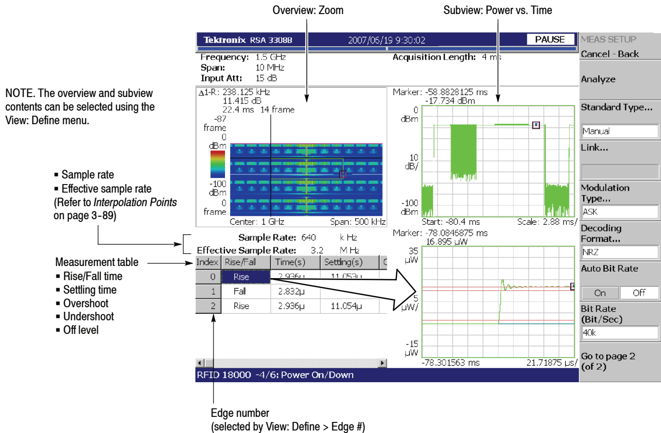
Figure 3-69: Power on/down measurements
