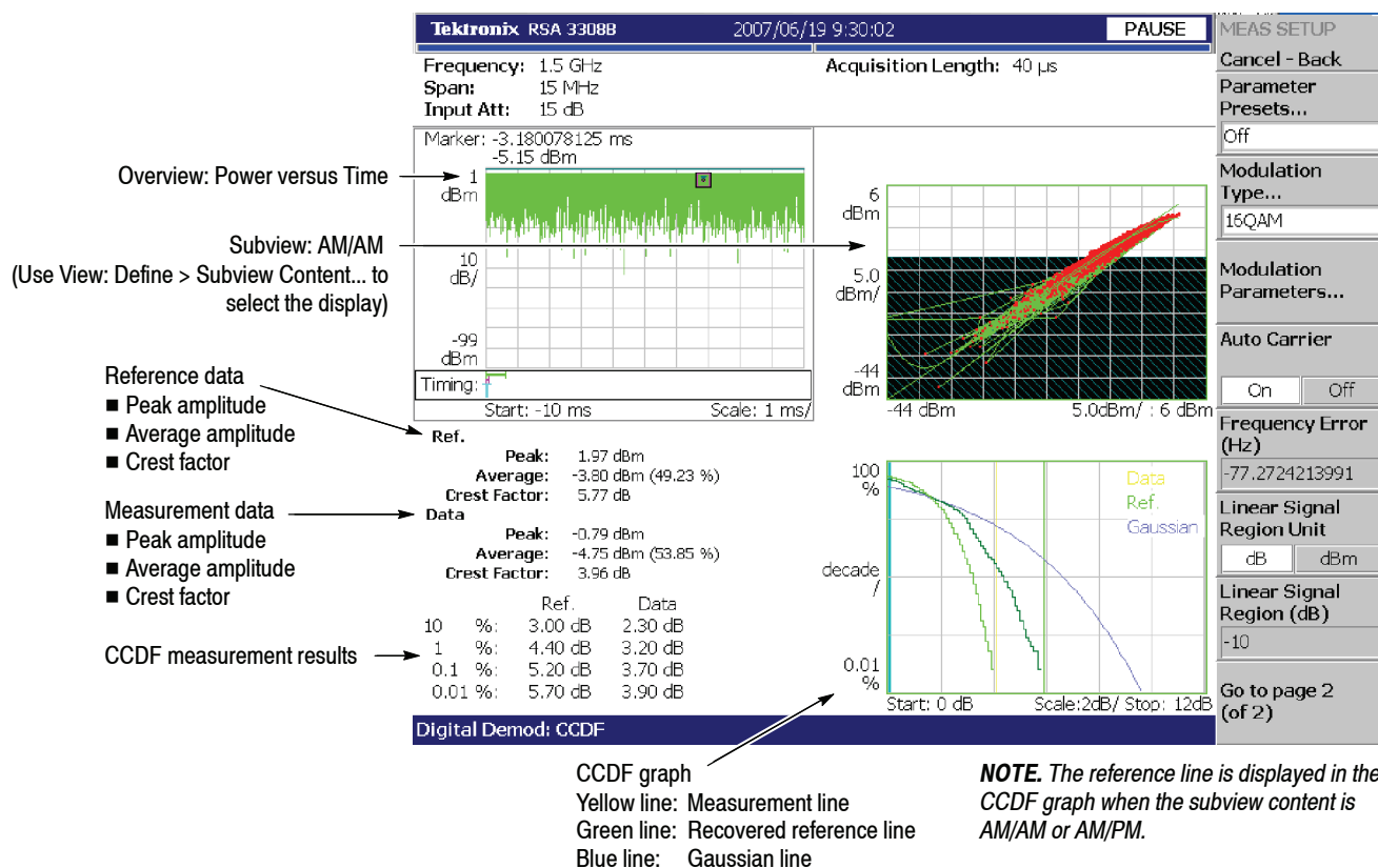
Figure 3-54: CCDF measurement
