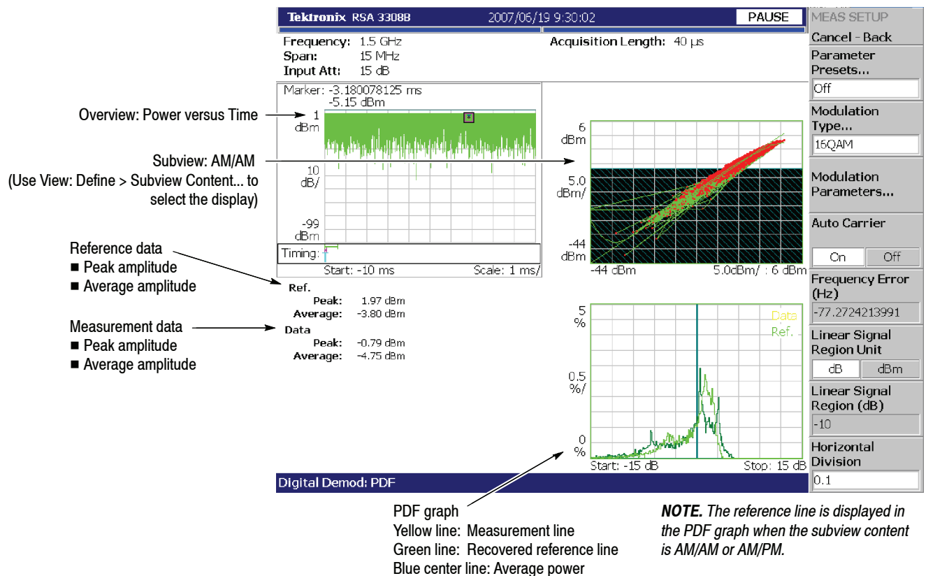
Figure 3-55: PDF measurement
