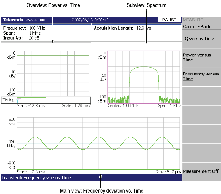
Figure 3-77: Frequency measurement
