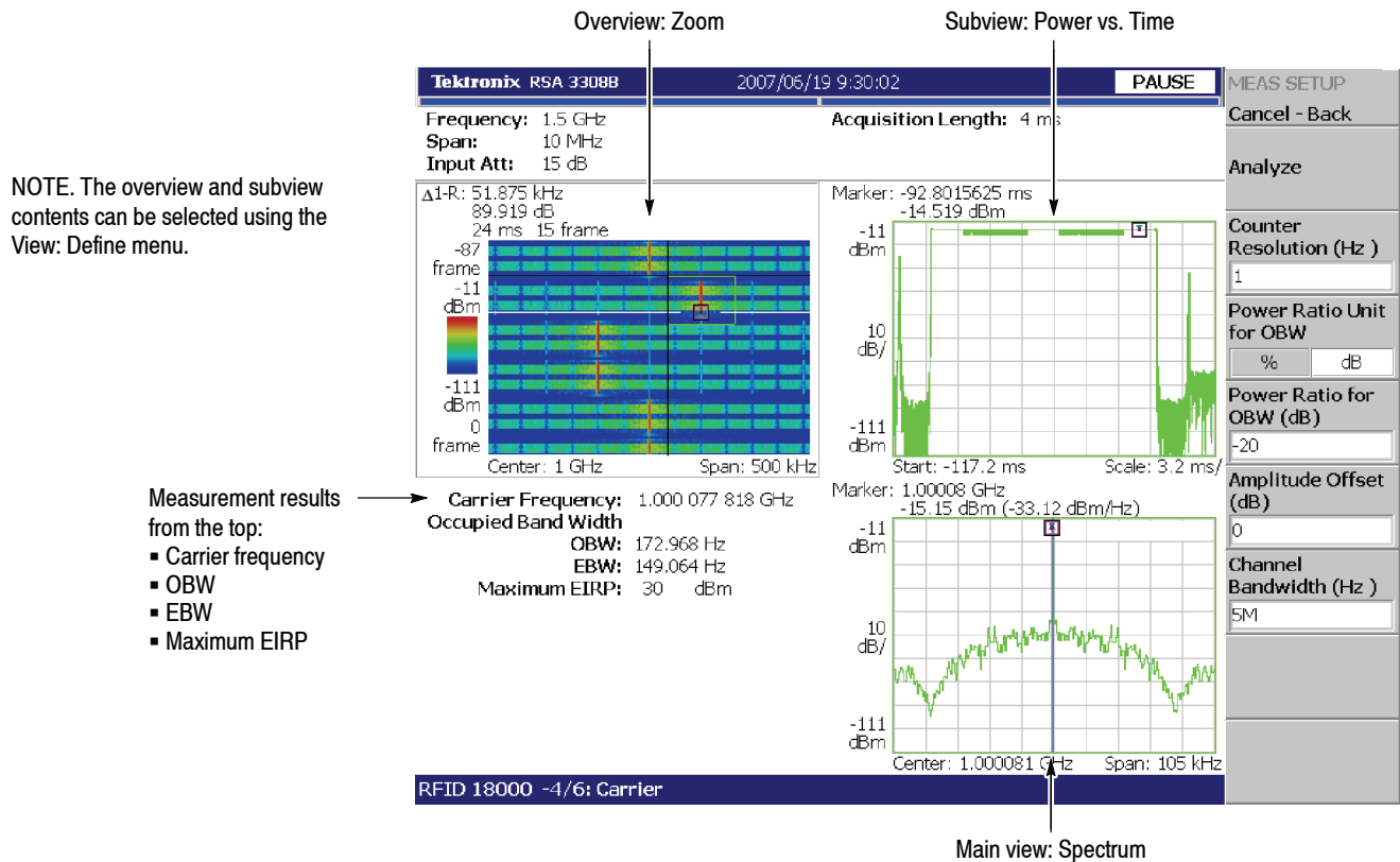
Figure 3-64: Carrier measurement
