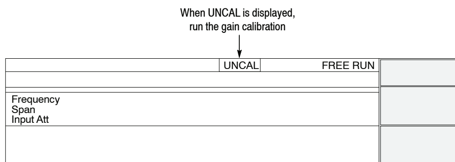
Figure 1-20: UNCAL display
