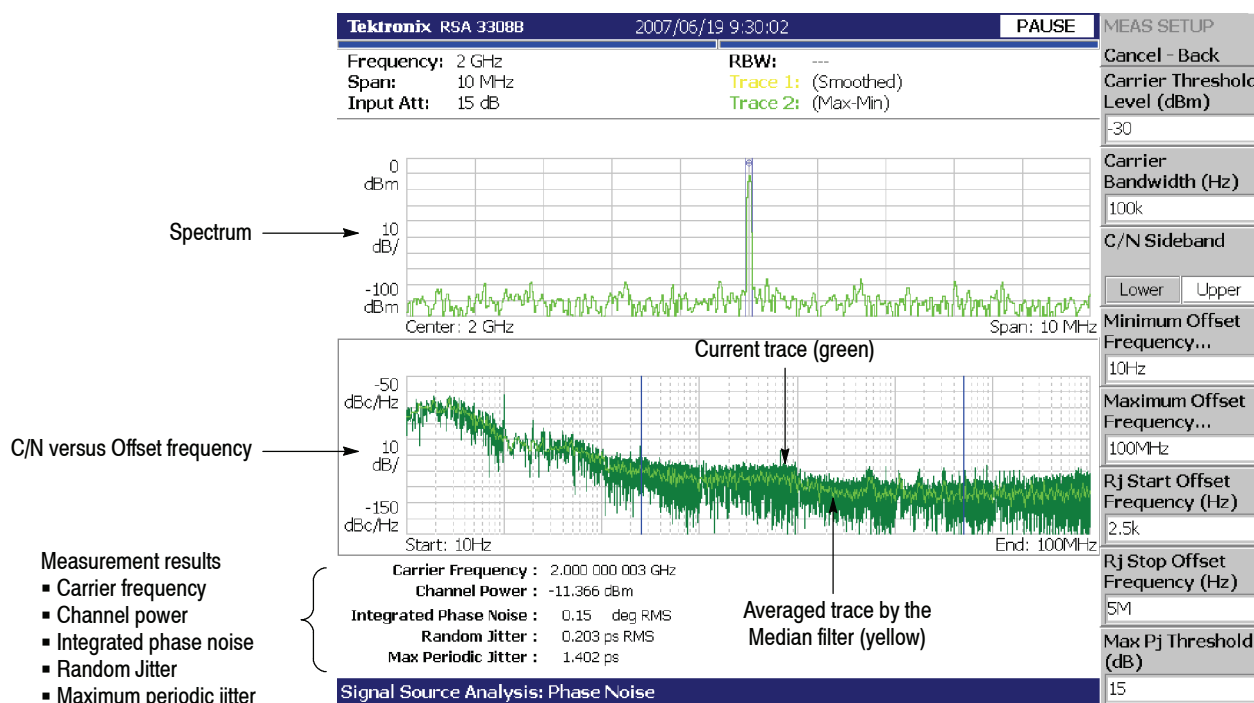
Figure 3-87: Phase noise measurement
