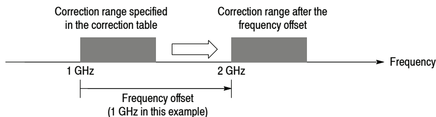
Figure 3-107: Frequency offset
