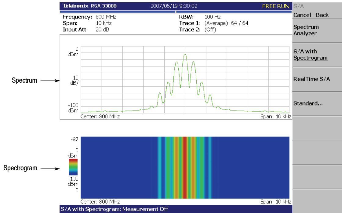
Figure 3-21: Spectrum and spectrogram concurrent display
