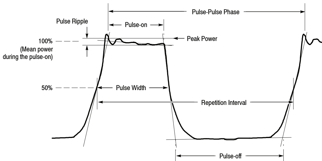
Figure 3-81: Definition of pulse characteristics
