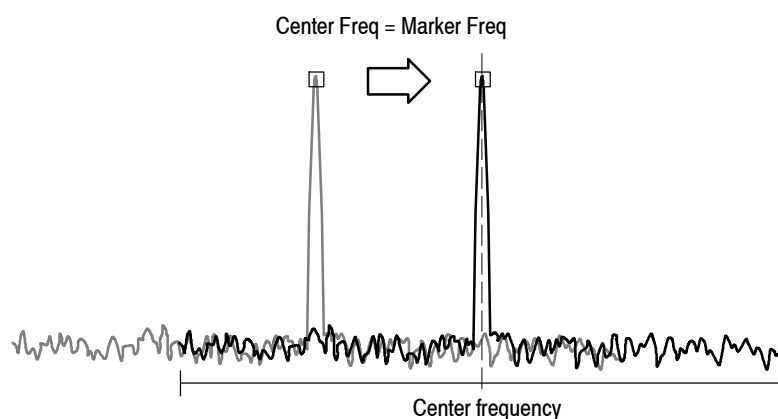
Figure 3-97: Setting the center frequency using Marker ➡
