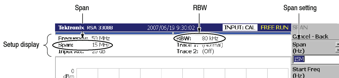
Figure 1-16: Setup display
