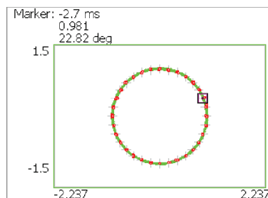
Phase Multiplication = x1, displaying 32 symbol points.
