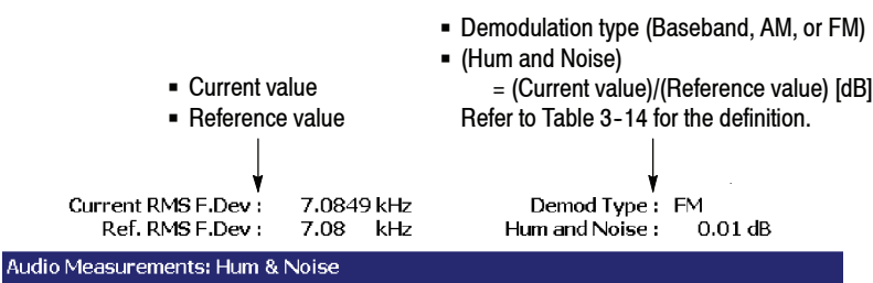
Figure 3-62: Hum and Noise Ratio measurement result (bottom of the screen)
