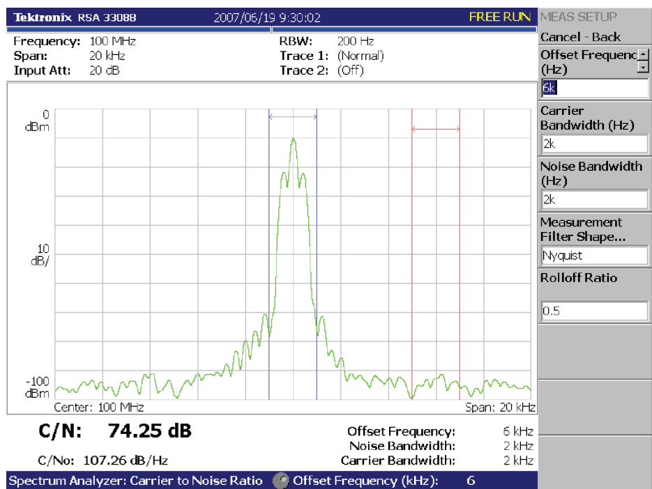
Figure 3-8: Example of C/N measurement
