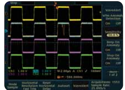
► WaveAlert waveform anomaly detection alerts you to any waveform that deviates from the "normal" input, such as the glitch on channel 2.
