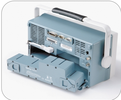
► TDS3BAT – Battery pack being installed. The TDS3000B oscilloscope weighs only 5.2 kilograms with battery pack.
