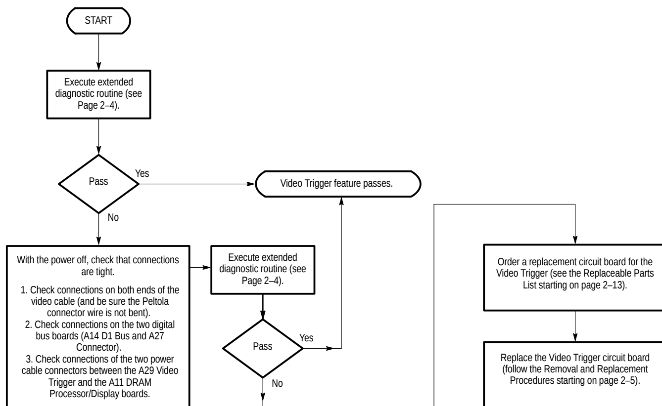
Figure 2–1: Troubleshooting Tree
