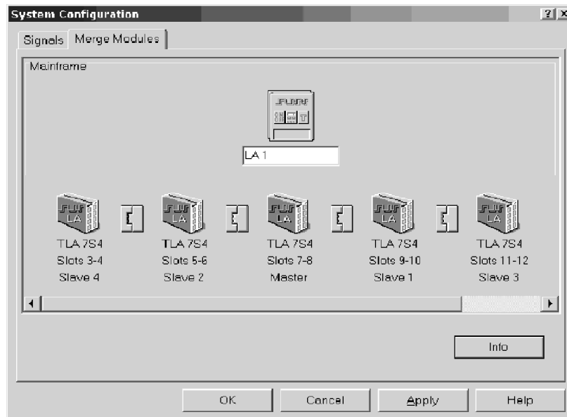
Figure 3-51: Merging modules
