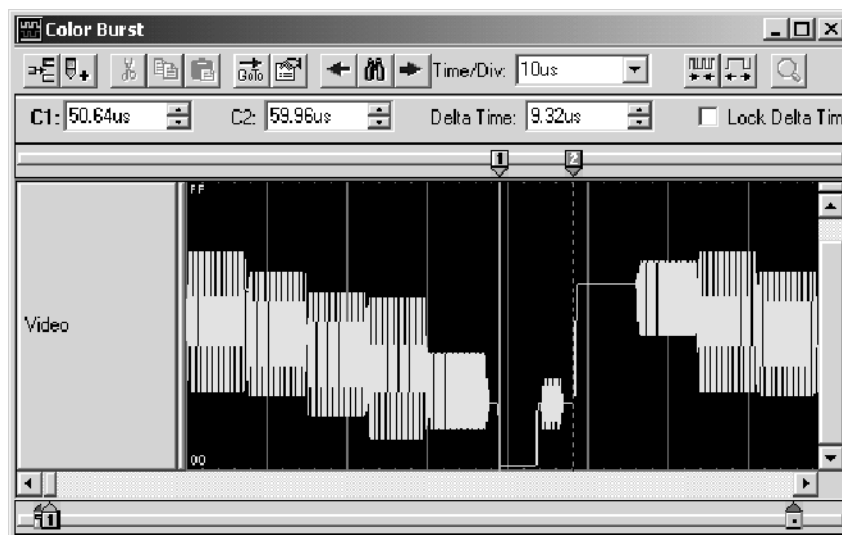
Figure 3-63: Magnitude waveform
